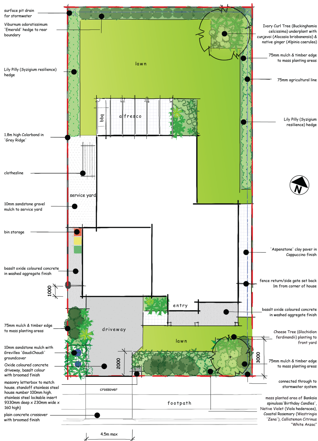
FIGURE 1: EXAMPLE LANDSCAPE PLAN
